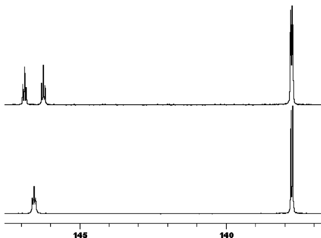
Figure 2. ^{13}\text{C} (top) and ^{13}\text{C}\{^1\text{H}\} (bottom) NMR spectra of ([\text{CN})_3\text{Pd}(\text{H})]^{2-} ( J_{\text{C-C}} = 5.8 Hz; \text{trans-}J_{\text{C-H}} = 64.9 Hz, \text{cis-}J_{\text{C-H}} = 2.6 Hz) in \text{CD}_3\text{CN} .
