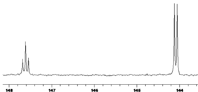
Figure 5. ^{13}\text{C}\{^1\text{H}\} NMR spectrum of [^{13}\text{CN}_3\text{PdBu}]^{2-} ( J_{\text{C-H}} = 6.8 \text{ Hz} ) in \text{THF-}d_8 .
