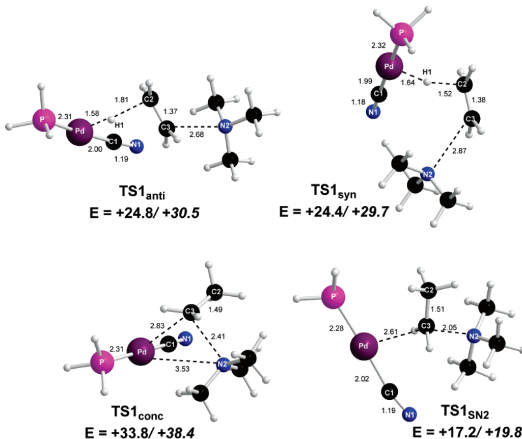
Figure 9. Computed transition state geometries for C–N activation in the [(\text{PH}_3)\text{Pd}(\text{CN})]^- \cdot [\text{Me}_3\text{NEt}]^+ ion pair ( 1 ) with selected distances in Å. Energies (kcal/mol) are given relative to 1 for the gas phase (plain text) and in THF solution (italics).
