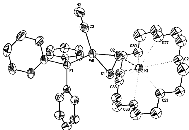
Figure 7. ORTEP drawing of [K·18-crown-6] + [(Ph 3 P) 4 Pd(CN)(O 2 )] - with thermal ellipsoids drawn to the 50% probability level. Selected bond distances (Å) and bond angles (deg): Pd(1)–C(2) 1.981(6), Pd(1)–O(1) 1.990(3), Pd(1)–O(2) 2.016(3), Pd(1)–P(1) 2.253(1), O(2)–O(1) 1.441(4), O(2)–K(1) 2.697(3), O(1)–K(1) 2.784(3), C(2)–Pd(1)–O(1) 154.6(2), C(2)–Pd(1)–O(2) 112.5(2), O(1)–Pd(1)–O(2) 42.2(1), C(2)–Pd(1)–P(1) 93.5(1), O(1)–Pd(1)–P(1) 111.9(1), O(2)–Pd(1)–P(1) 154.0(1), N(2)–C(2)–Pd(1) 177.4(5).
