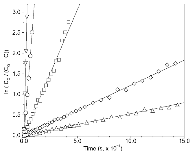
Figure 6. First-order kinetic plot for the formation of [(^{13}\text{CN})_3\text{PdBu}]^{2-} at 5 °C ( \Delta ), 10 °C ( \diamond ), 20 °C ( \square ), 30 °C ( \circ ), and 40 °C ( \nabla ) in THF- d 8 . Data acquisition at 5 °C was continued out to 65.6 h.
