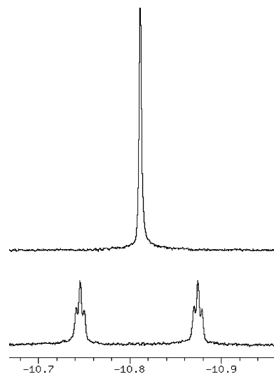
Figure 1. ^1\text{H} (bottom) and ^1\text{H}\{^{13}\text{C}\} (top) NMR spectra of ([\text{CN})_3\text{Pd}(\text{H})]^{2-} ( \text{trans-}J_{\text{C-H}} = 64.9 Hz, \text{cis-}J_{\text{C-H}} = 2.6 Hz) in \text{CD}_3\text{CN} .
