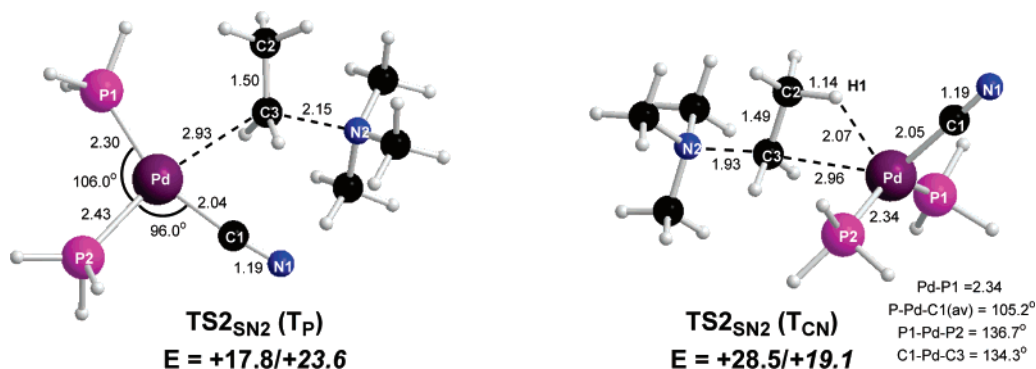
Figure 12. Computed S N 2 transition states for C–N activation in [(PH 3 ) 2 Pd(CN)] − ·[Me 3 NEt] + ( 2 ) with selected distances (Å) and angles. Energies (kcal/mol) are given relative to 2 for the gas phase (plain text) and in THF solution (italics).
